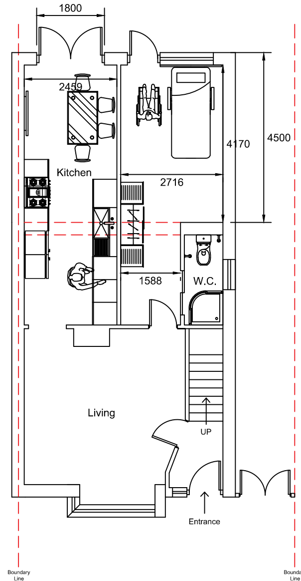
Proposed Ground Floor 1
