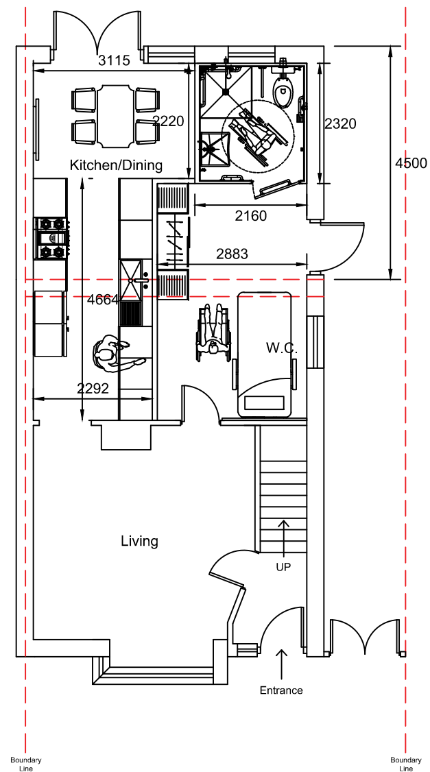
Proposed Ground Floor 2
